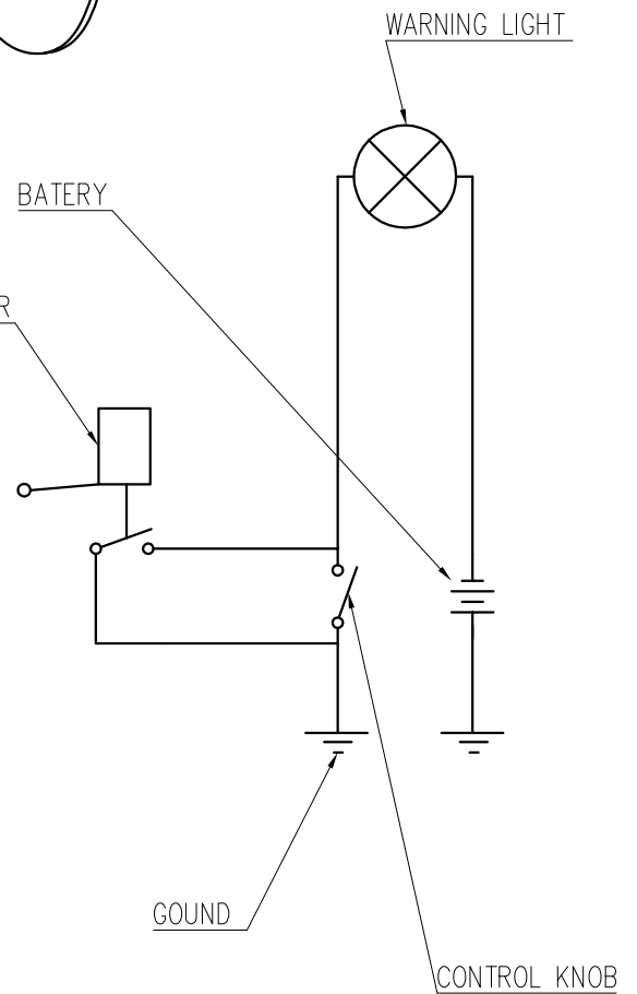
WIRING SCHEMA OF FUEL SENSOR
